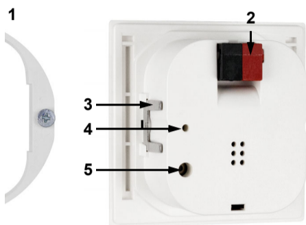
Fig. 2: Rear
