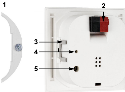
Fig. 3: Rear
