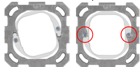
Fig. 4 Hook the mounting adapter into the mounting plate of the switch system and tighten the screws.
