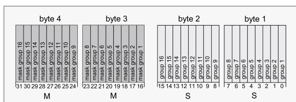
Figure 13: Structure of the objects of the collective feedback, using the example of the object for Groups 1-16
