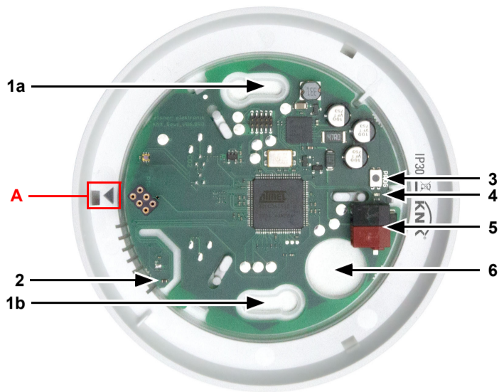
Fig. 1 1 a+b Long holes for mounting (hole distance 60 mm) 2 Sensor for temperature 3 Programming button 4 Programming LED 5 KNX-terminal BUS +/- 6 Cable bushing A Mark for aligning the cover
