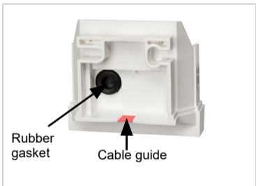
Fig. 10 Break the cable guide off. Feed the power lead through the rubber gasket.
