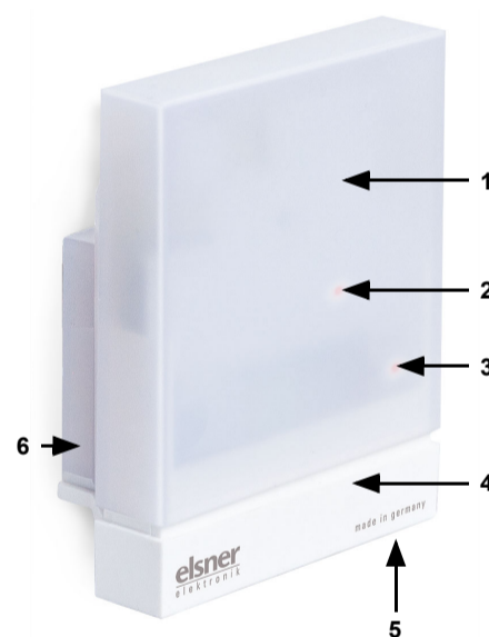
Fig. 3 1 Semi-transparent cover (GPS receiver below) 2 Position of the Signal LED (under the cover). LED is freely controlled via two objects 3 Position of the programming LED (under the cover) 4 Lower part of housing 5 Programming key on the bottom of the housing (recessed), see "Device design" auf Seite 1 6 Wall/Pole holder
